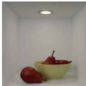
▲ Neutral white (NW) - 4,200 kelvin (3 Vdc / 0.7A = 130 lumen)
