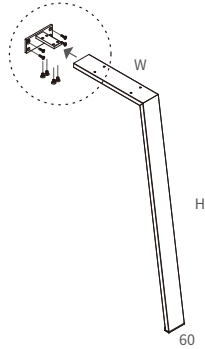
AFT6-WW Wall-Mounted J Leg *Height: 410, 700 & 850mm
