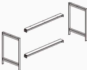
Frame High Leg, with 2 cross beams
