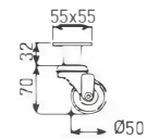
ZPT-AKE50BKB-220BKB (with brake)
