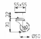
ZPT-AKE50ABN-220BNB (with brake)
